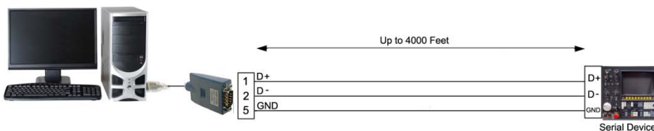
Connection example: extending communication distance with RS485
